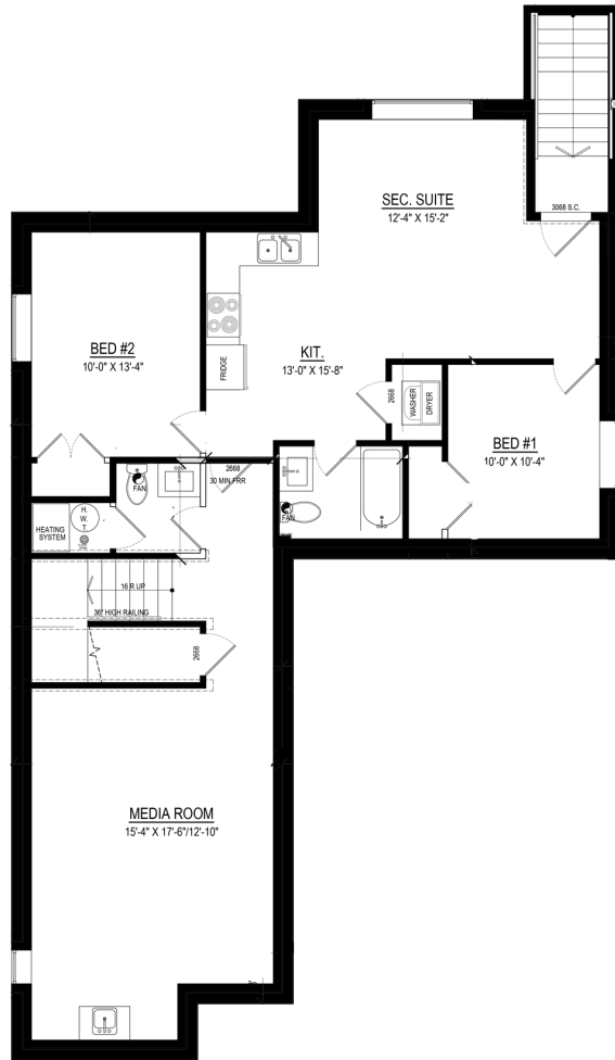
Basement 1750 sq. ft.
